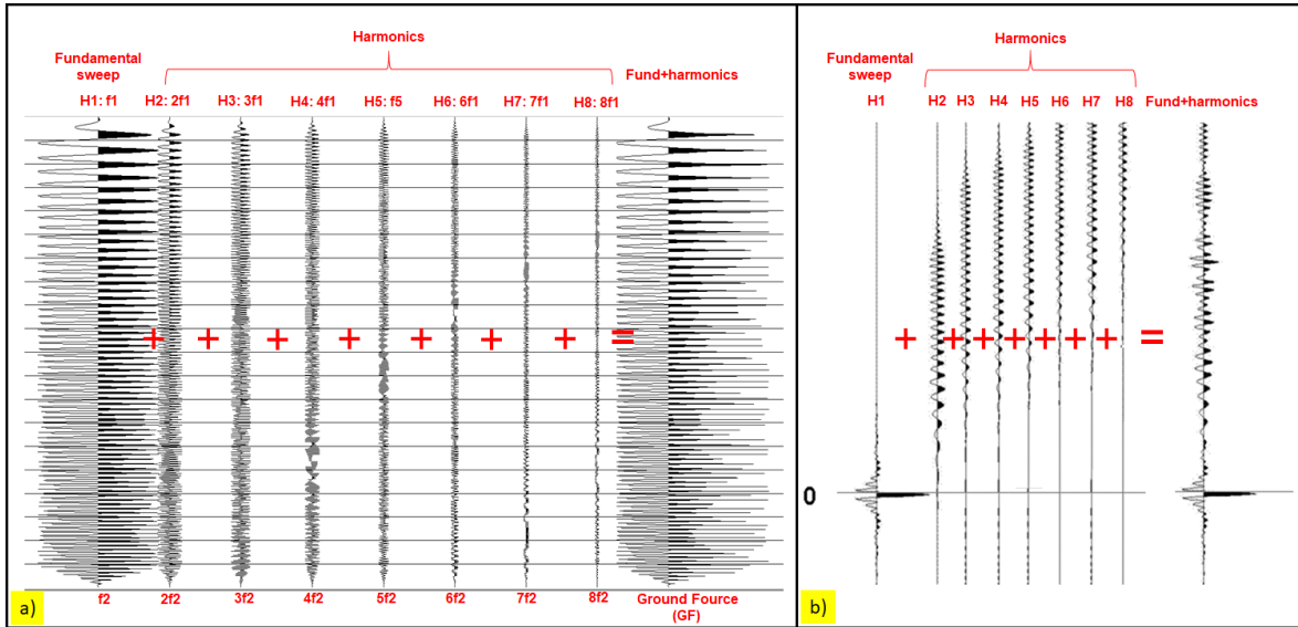
Figure-7: a) A synthetic fundamental sweep and its eight harmonics, b) A cross-correlation of fundamental sweep and its eight harmonics with fundamental sweep and their summing.
