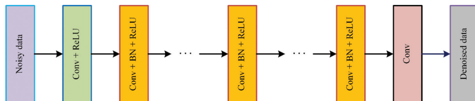
Figure 1. Structure of a denoising convolutional neural network.
