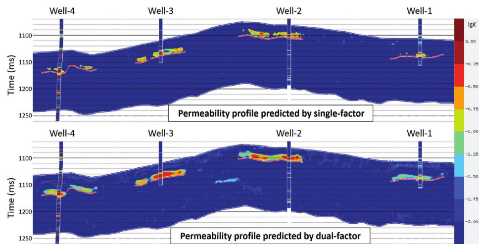
Figure 4. Predicted permeability profiles, where dual-pore-structure parameters refer to c_{\mu}+\alpha and single-factor denotes \gamma_{\mu} . Reprinted with permission from Ding et al. 39 Copyright 2023 Society of Exploration Geophysicists.
