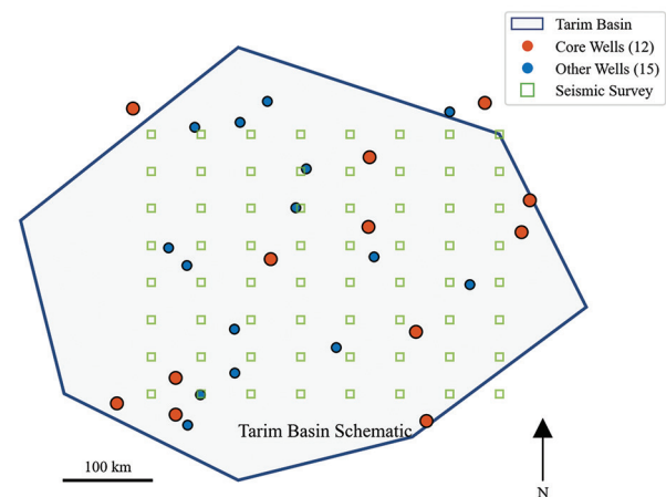
Figure 5. Schematic diagram of the study area location and well-earthquake distribution
