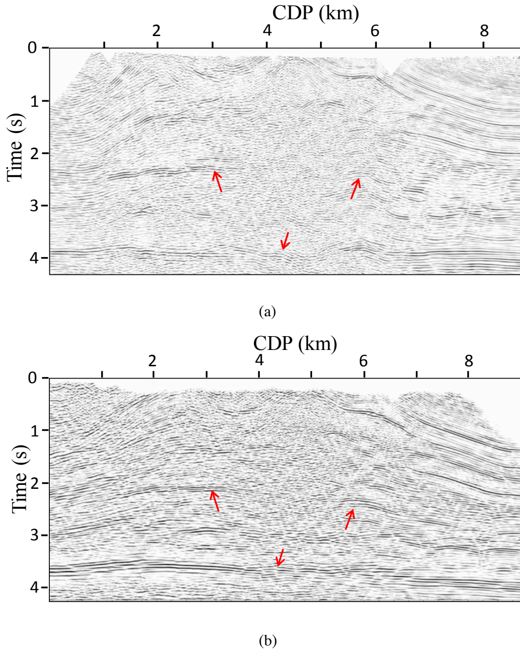
Fig. 12. Comparison of PSTM between wide line data (a) and swath 3D data (b).
